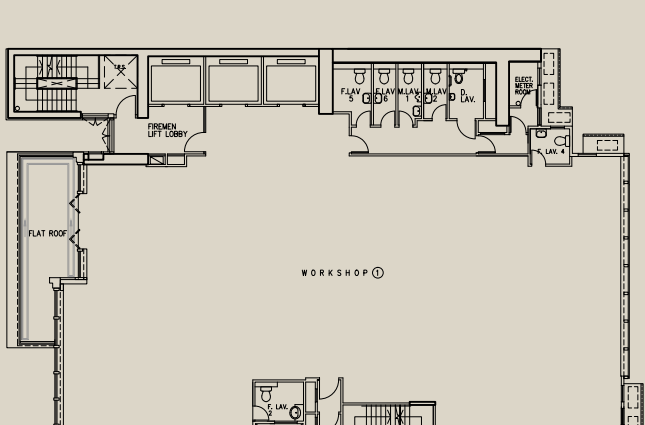
19F + FLAT ROOF 6,635 SQ. FT.
