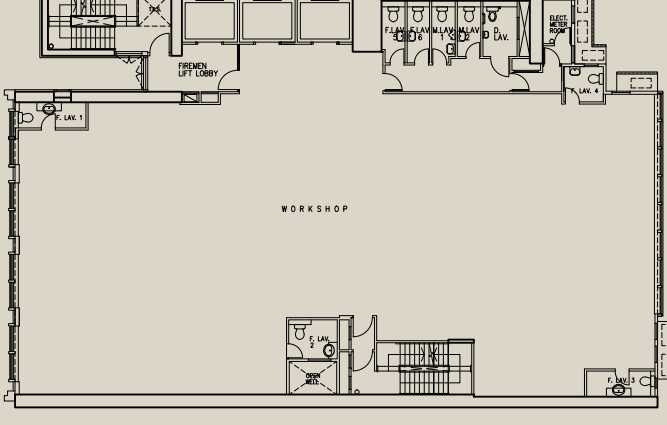
5F 7,734 SQ. FT.
